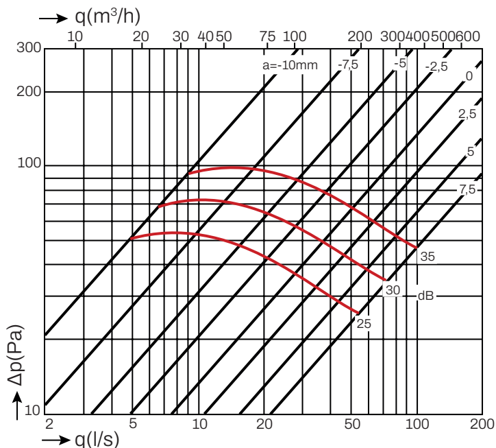
SUPPLY Ø150
