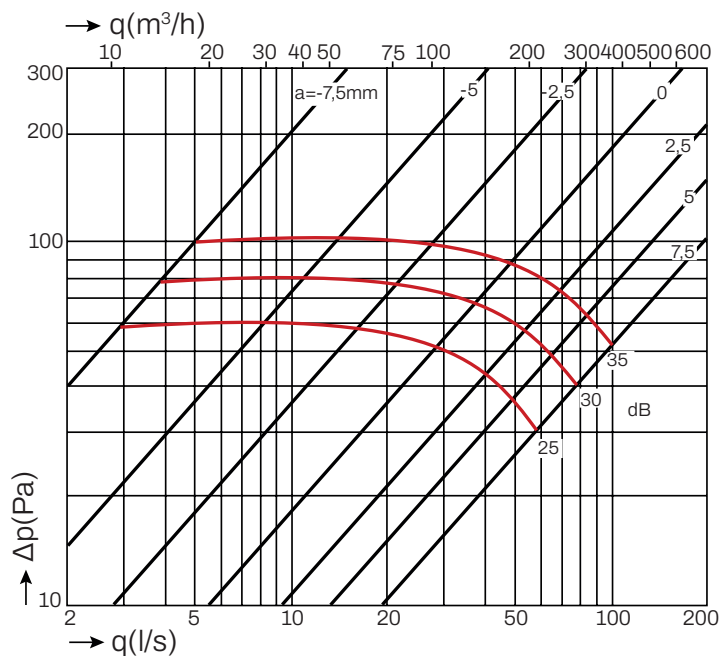
SUPPLY Ø160
