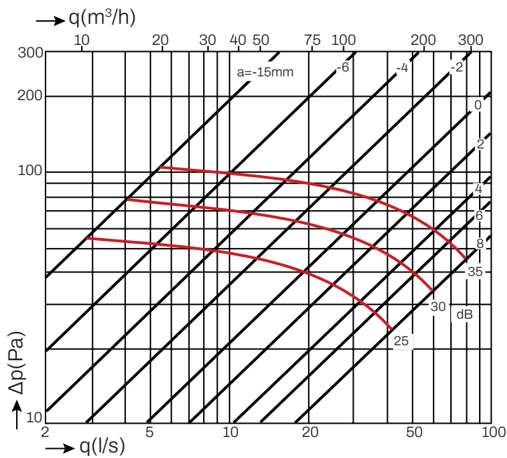
SUPPLY Ø150
