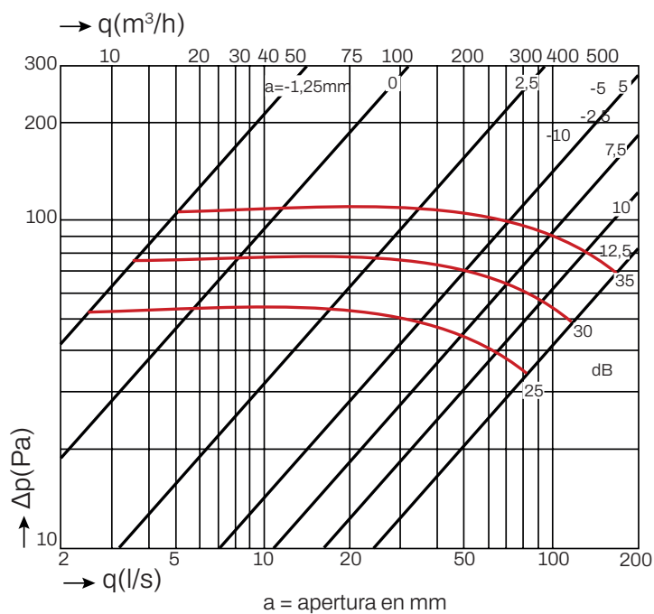
SUPPLY Ø200
